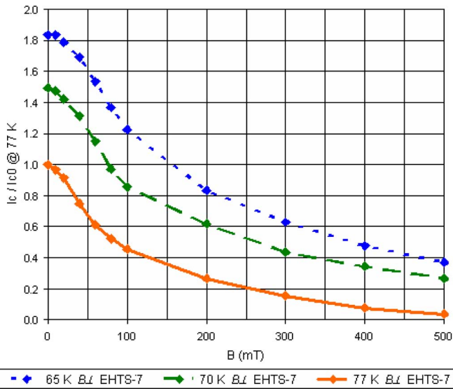
Fig. 5. I_c(B) measurements performed on EHTS-7 stack at 65 K, 70 K and 77 K and in perpendicular field ( B \perp ). Measured I_c values are normalized to I_c at 77 K s.f. (340 A).
