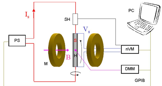
Fig. 1. Sketch of set-up used for critical current vs magnetic field measurements. The sample and the magnet were immersed in the same liquid nitrogen bath.
