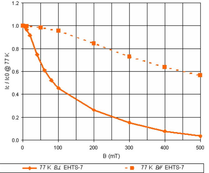
Fig. 3. I_c(B) measurements performed on EHTS-7 stack at 77 K in parallel ( B \parallel ) and perpendicular ( B \perp ) field. Measured I_c values are normalized to I_c at 77 K s.f. (340 A).
