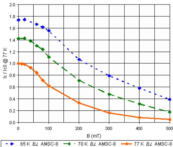
Fig. 6. I_c(B) measurements performed on AMSC-8 stack at 65 K, 70 K and 77 K and in perpendicular field ( B \perp ). Measured I_c values are normalized to I_c at 77 K s.f. (650 A).
