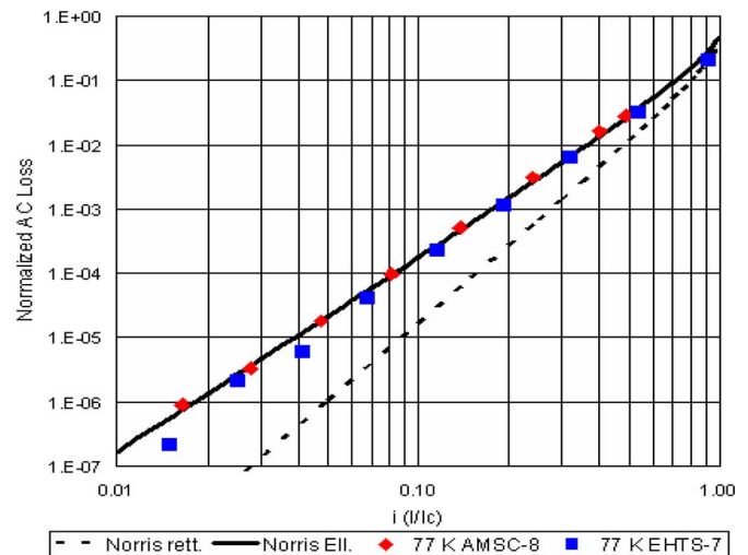
Fig. 7. Transport AC loss measurements performed on EHTS-7 and on AMSC-8 stacks at 77 K compared with Norris losses. Measured losses (W/m) are normalized to f\mu_0 I_c^2/\pi .
