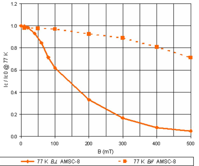
Fig. 4. I_c(B) measurements performed on AMSC-8 stack at 77 K in parallel ( B \parallel ) and perpendicular ( B \perp ) field. Measured I_c values are normalized to I_c at 77 K s.f. (650 A).
