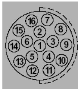
Fig.2 - Schematic of DEE 104 A086 instrumentation connector ( seen underside )
