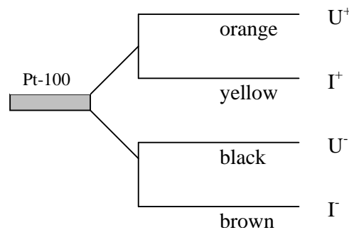
Fig.3 - Schematic of Pt-100 probe and instrumentation wires
