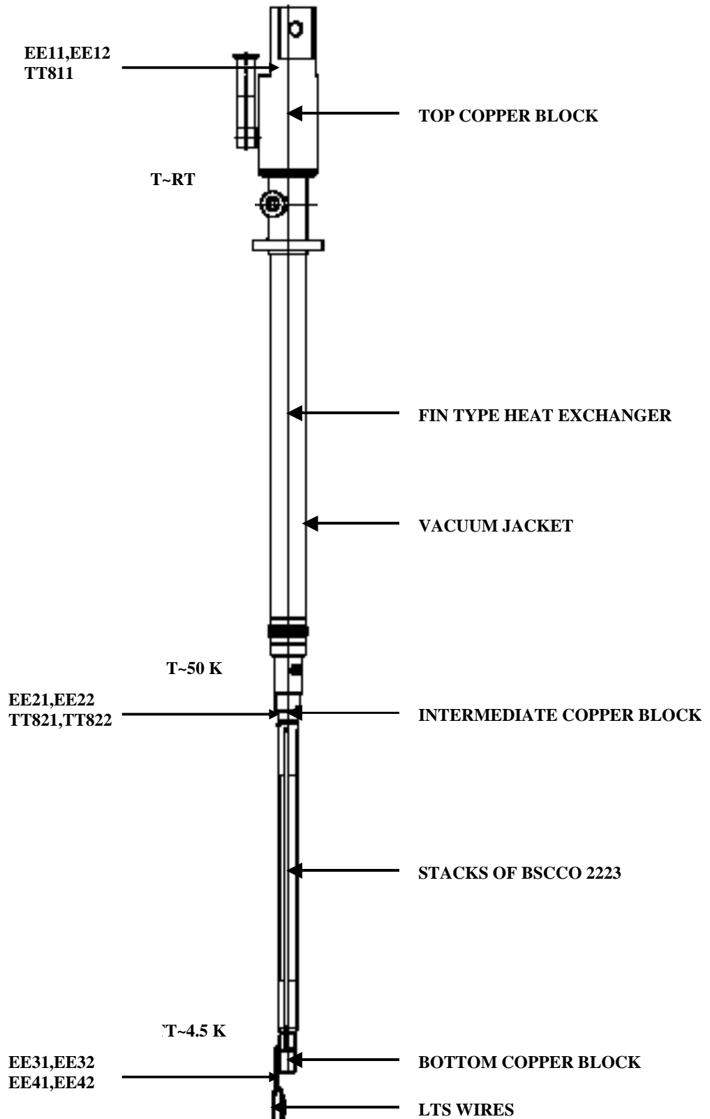
Fig. 1 - 600 A HTS current lead schematic
