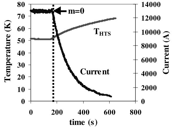
Fig. 6. Increase of T_{HTS} during a 20 K helium coolant loss measurement.
