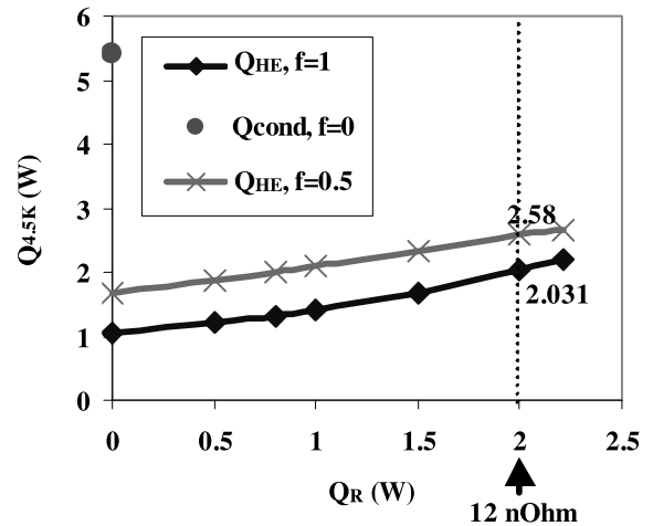
Fig. 4. Heat load at 4.5 K as a function of power dissipation of cold joint of HTS.
