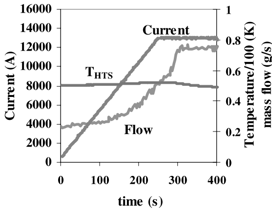
Fig. 5. Measured time dependence of current, T_{HTS} and 20 K helium flow during a ramp from 0 to 13000 A, with temperature control of the helium flow.
