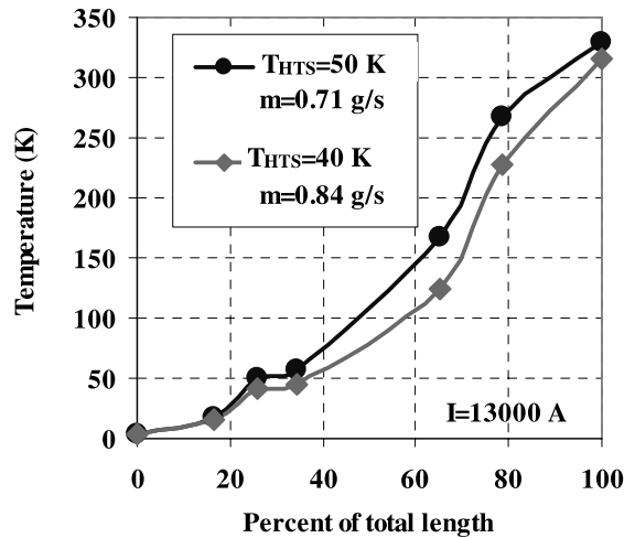
Fig. 3. Measured temperature profile of prototype lead (temperature as function of % of total lead length).
